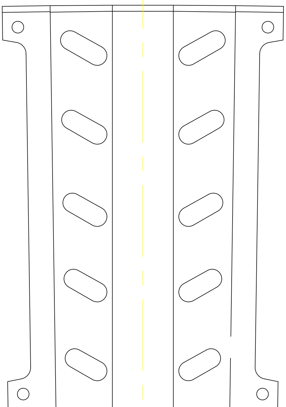
Fwd Heat Shield Flat Pattern
